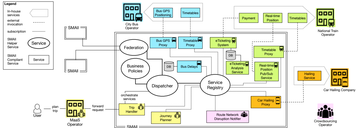
Fig. 1. Example of the SMALL architecture.
