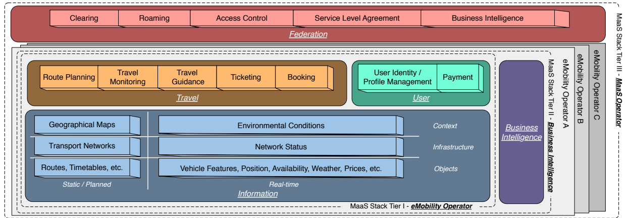
Fig. 2. The MaaS Stack
